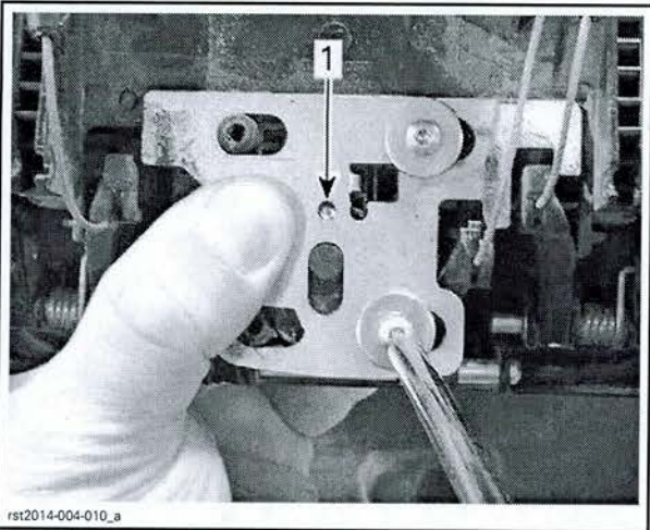
1. Ball and spring location under cam plate
