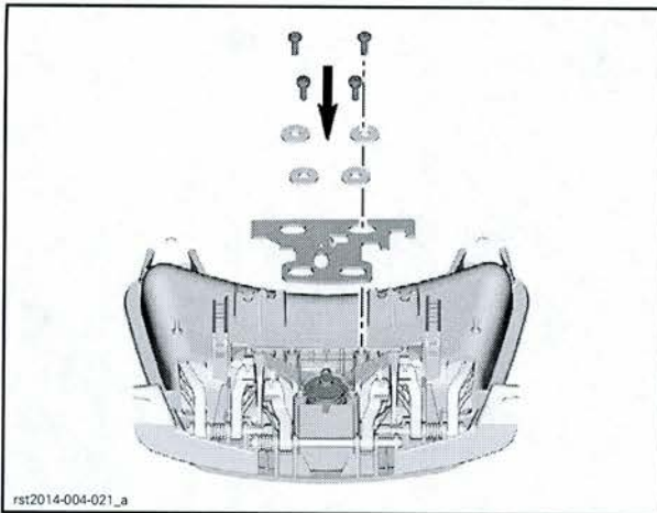
CAM PLATE INSTALLATION
