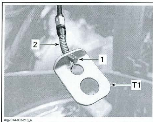
T1 INSERTION ON CABLE END
