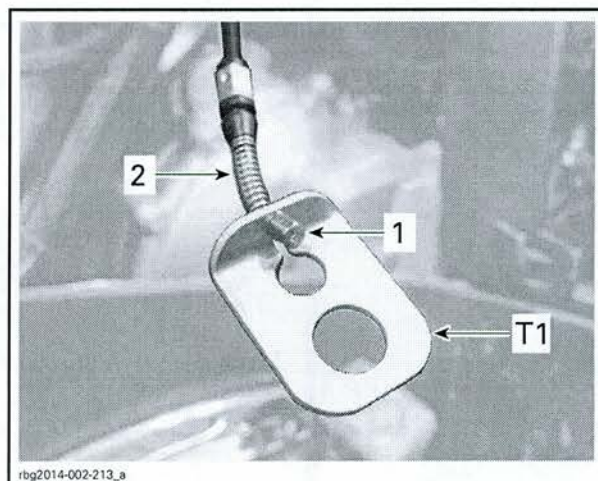
RS AND ST MODELS 1. Cable end 2. Spring
