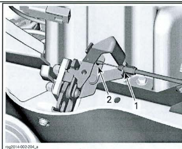
STORAGE COMPARTMENT LATCH (RT MODEL) 1. Cable retainer 2. Latch pivot plate
