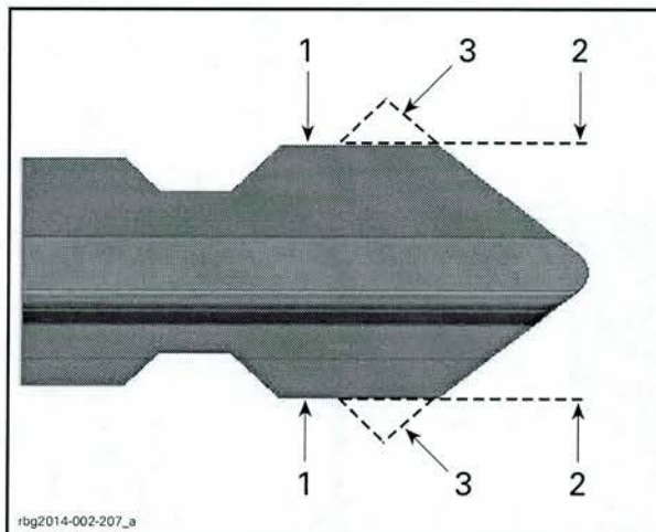
1. Reference flat surface 2. Cut line 3. Material removed
