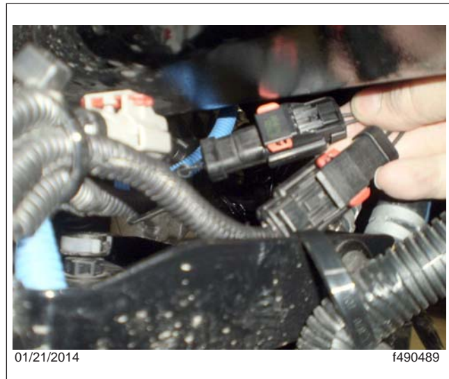
Fig. 5, Heater Connectors
