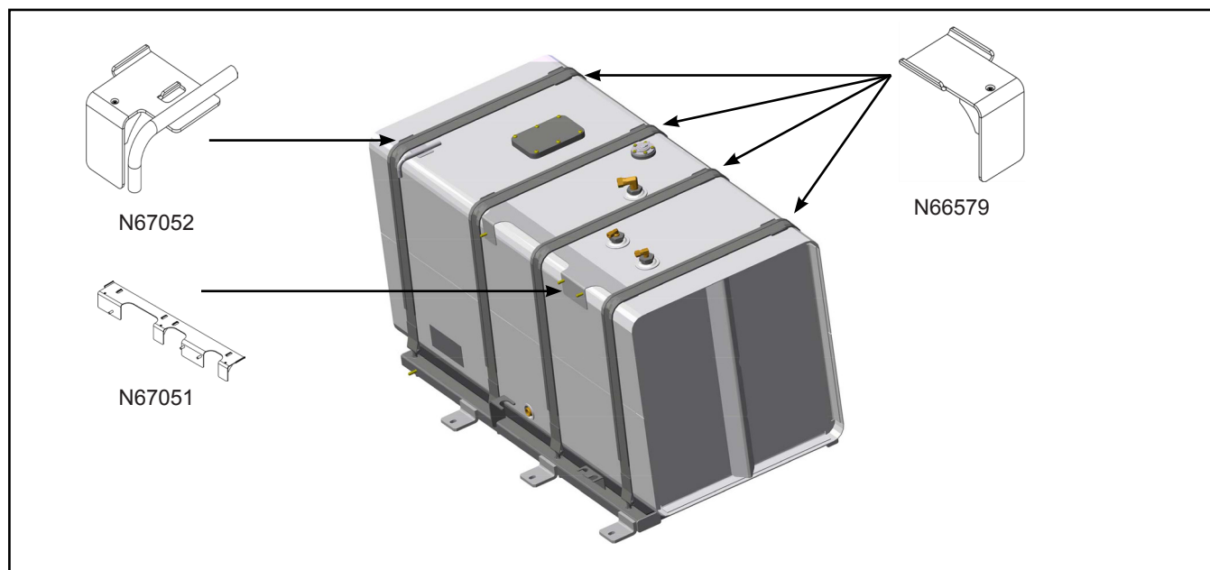
Figure 1 - Fuel Tank
