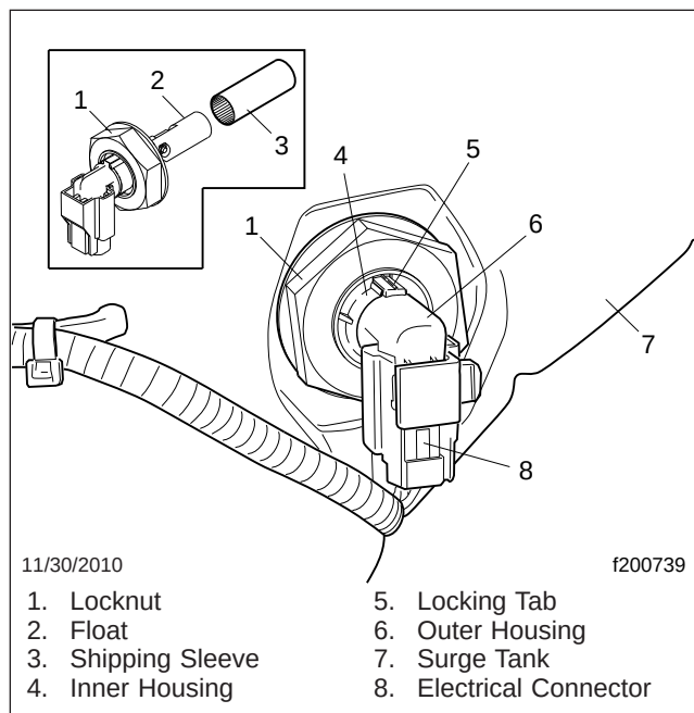
Fig. 2, low-coolant-level Sensor
