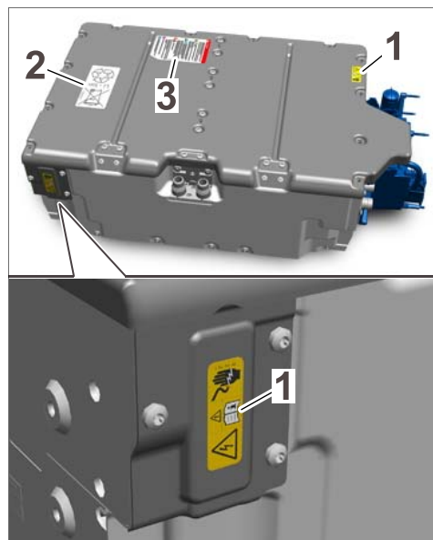
Arrangement of stickers
