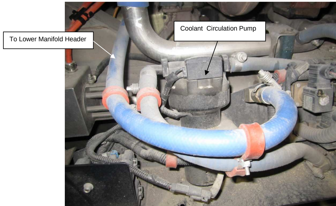
Figure 3: Hose Layout at Coolant Circulation Pump.
