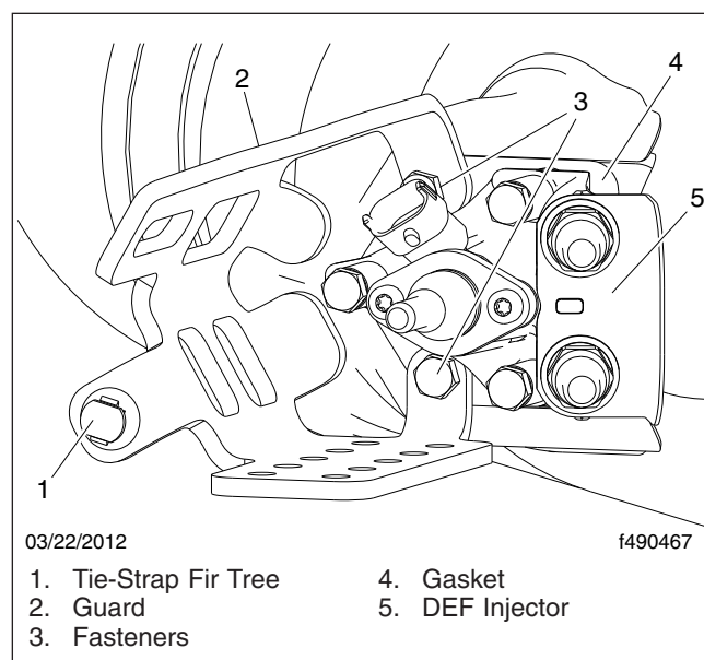
Fig. 1, Heavy-Duty Guard Installation (04-29937-000)
