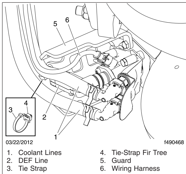
Fig. 3, Line and Wiring Harness Installation (04-29937-000)
