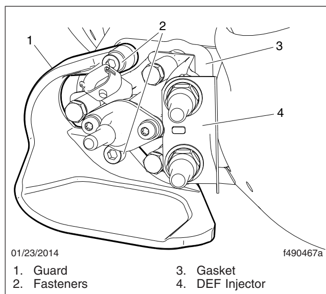
Fig. 2, Heavy-Duty Guard Installation (04-30694-000)
