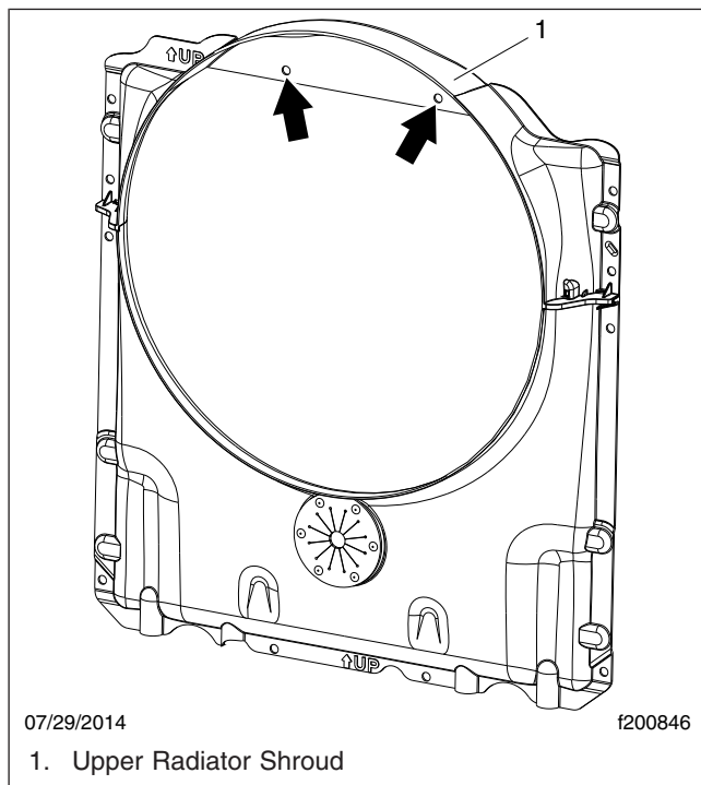
Fig. 1, Fastening Points
