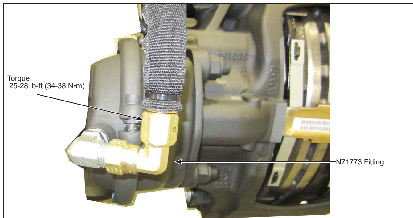
Figure 4 - N71773 Fitting Torque
