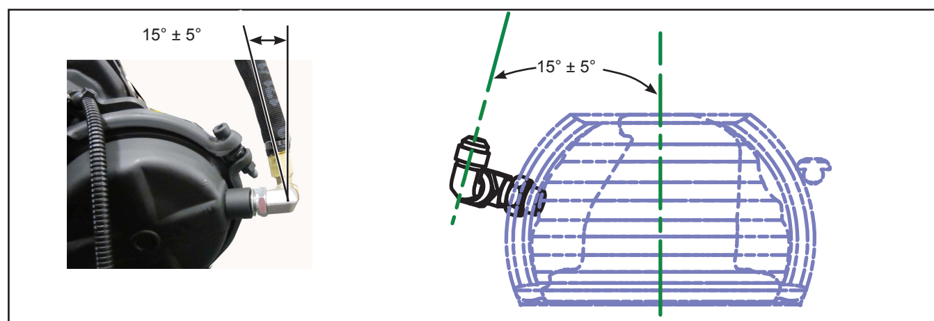
Figure 3 - N71773 Fitting Angle Positioning
