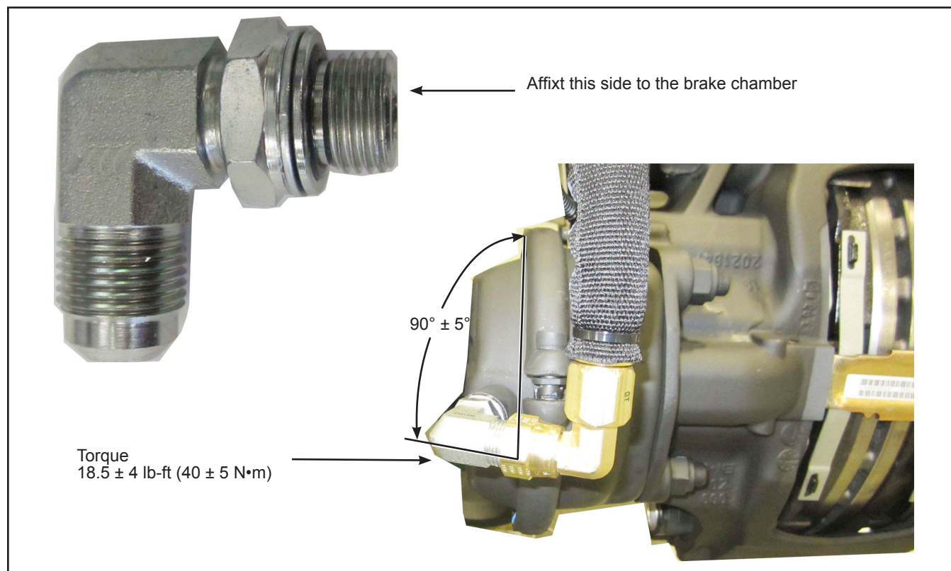
Figure 2 - Torque and Positioning of the N71772 Elbow
