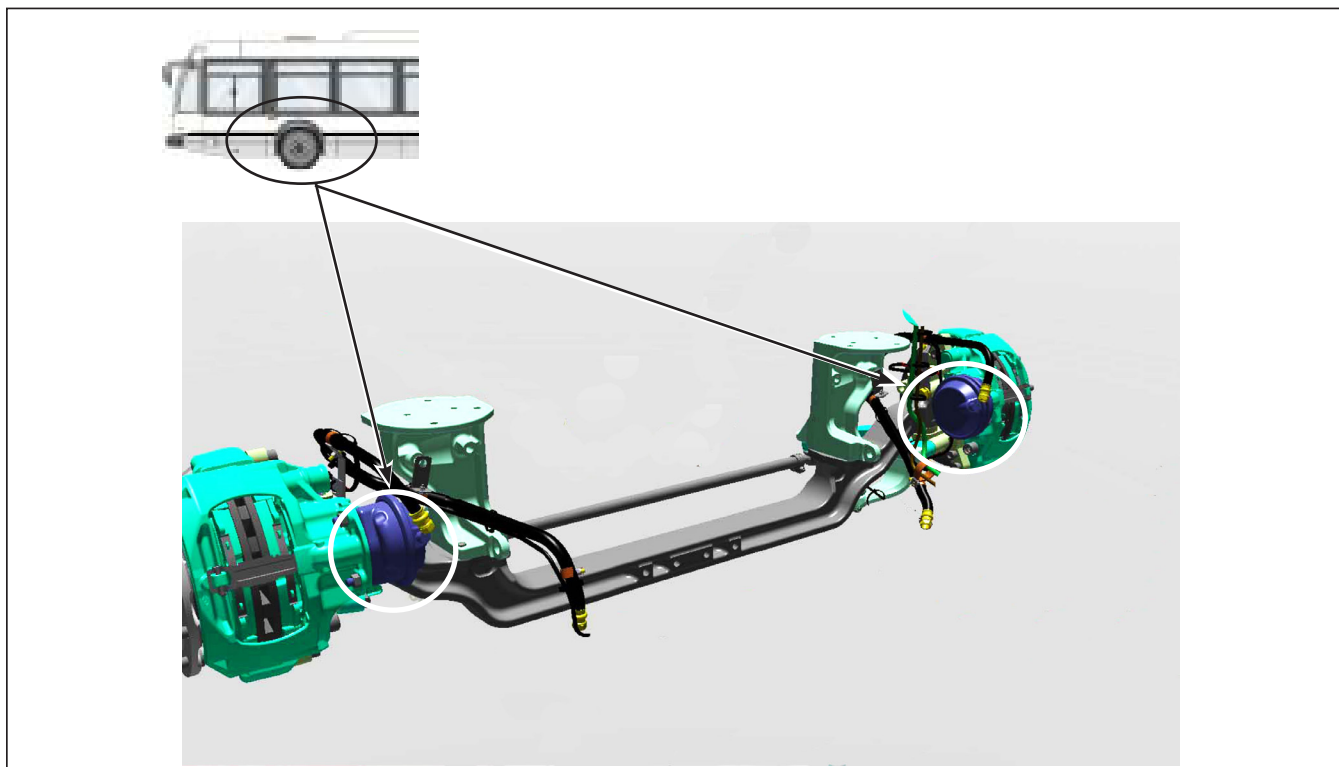
Figure 1 - Front Brake Chamber Location
