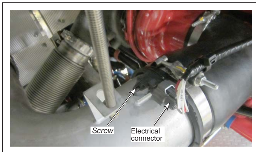
Figure 2 - Temperature/Pressure Sensor
