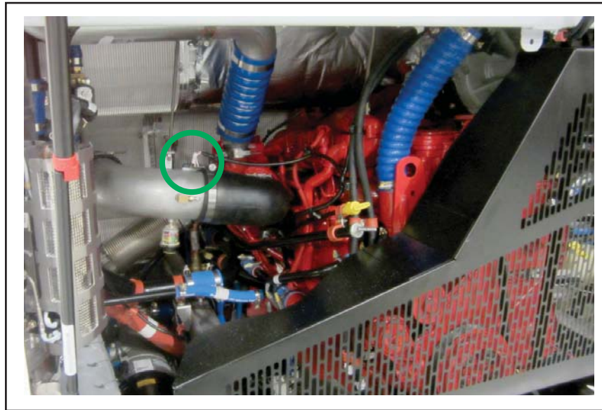
Figure 1 - Temperature/Pressure Sensor Location
