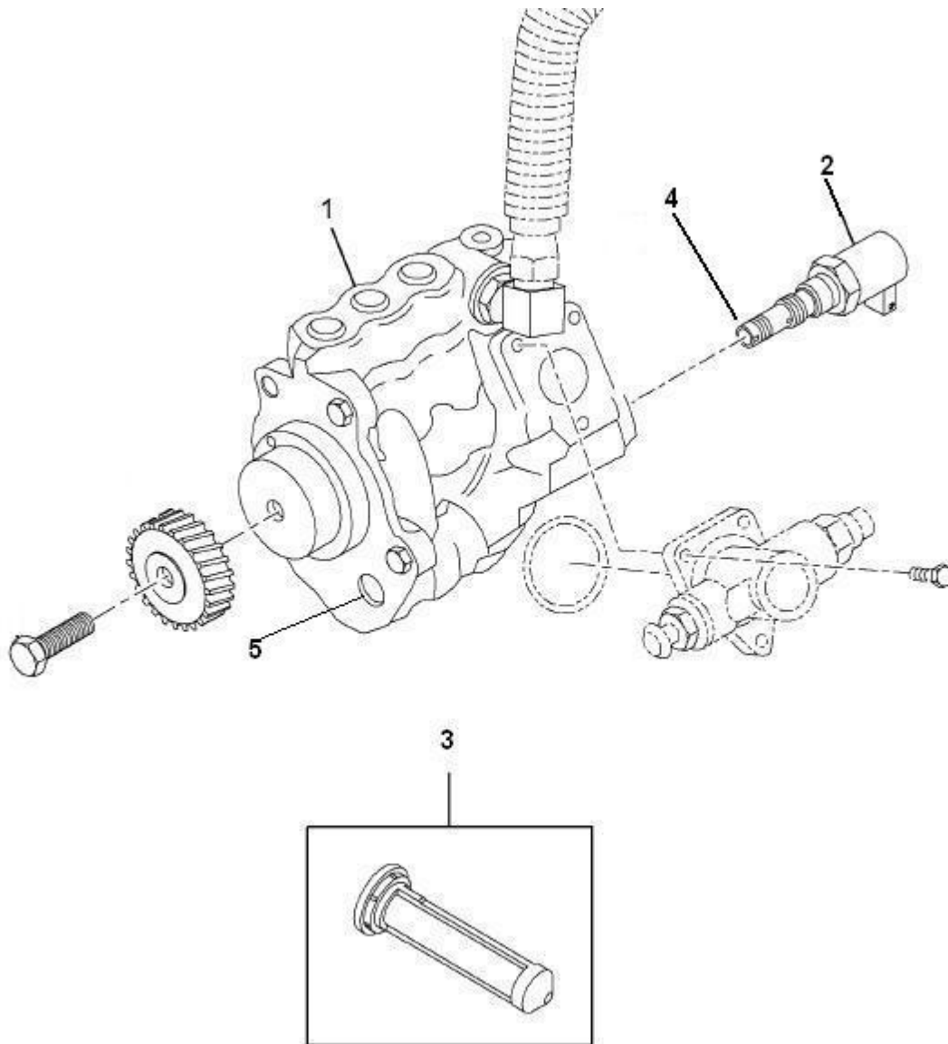
Figure 1: High Pressure Oil Pump
