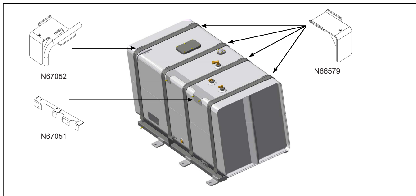
Figure 1 - Fuel Tank
