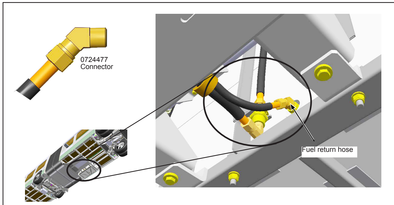
Figure 2 - 0724477 Connector for the Fuel Tank Return Hose
