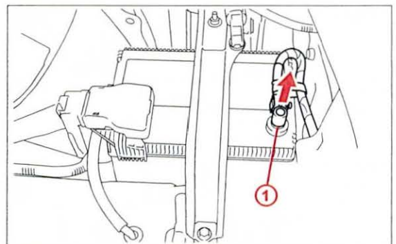
1 Negative Terminal
