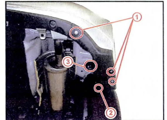
1 Self-Tapping Screws 2 Plastic Wing Nut 3 Plastic Retainer Clip
