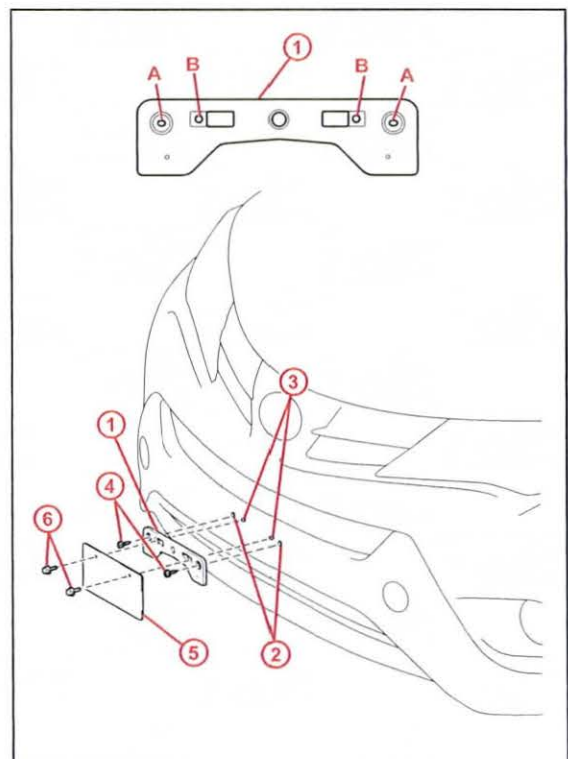
1 Mounting Bracket 2 Dimples 3 Mark and Drill Holes 4 Self-Tapping Screws 5 License Plate 6 Bolts
