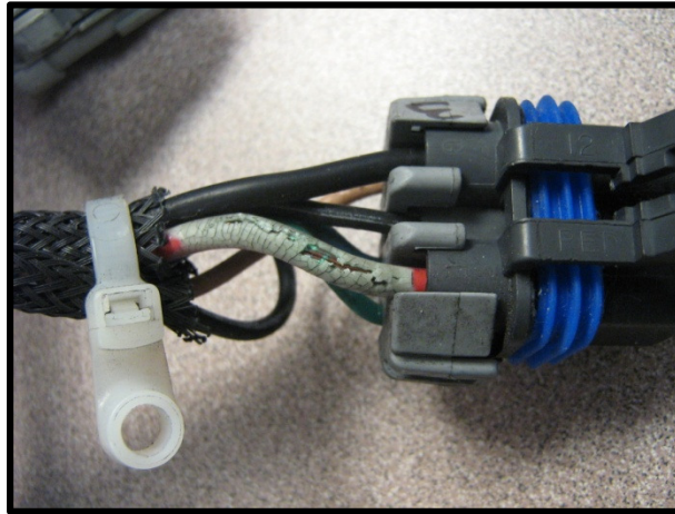
Figure 2: Main Harness Damage
