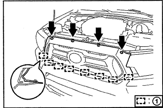
1 Guides
