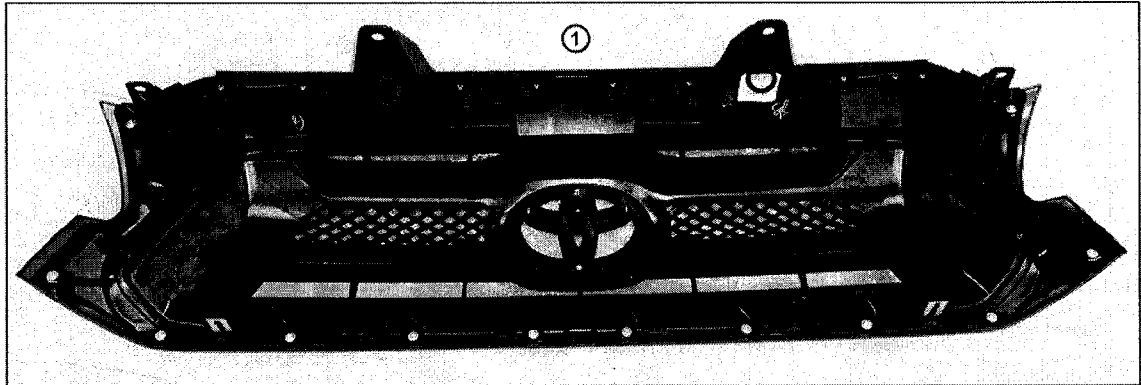
Figure 14. Back View of Radiator Grille
