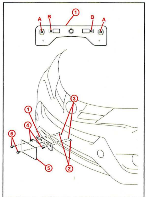
1 Mounting Bracket 4 Self-Tapping Screws 2 Dimples 5 License Plate 3 Mark and Drill Holes 6 Bolts
