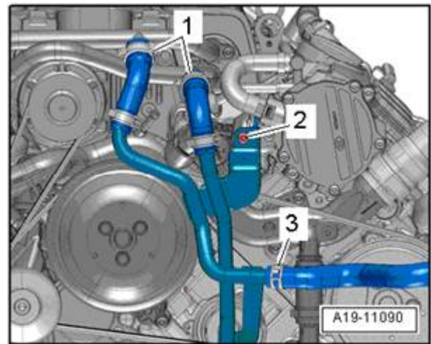
Figure 2. Front coolant pipes to be removed for 3.0T
