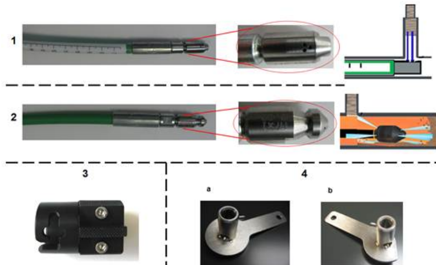
Figure 6. Special tool set VAS6825
