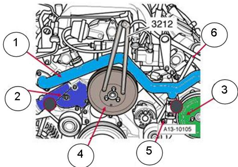
Figure 3. Engine component removal
