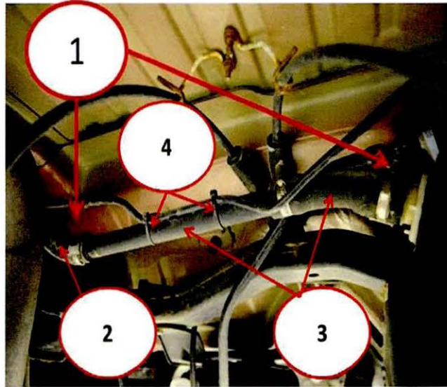
Fig. 1 Fuel Tubes
