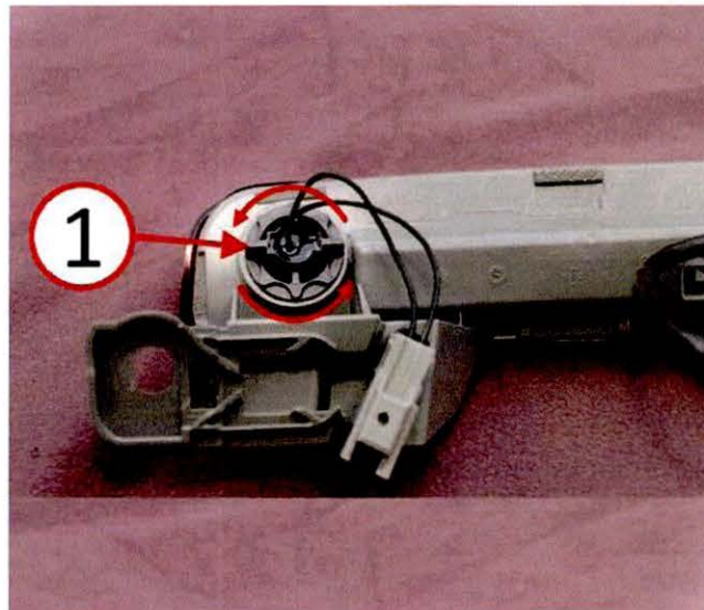
Fig. 3 Passive Entry Switch Removal
