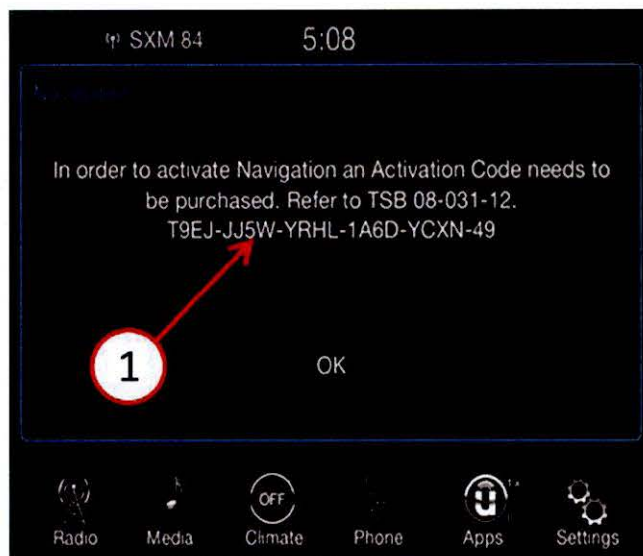
Fig. 2 Request code
