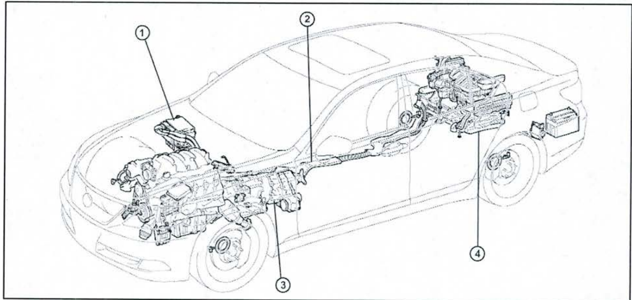
Figure 1. High-Voltage Components and Cables
