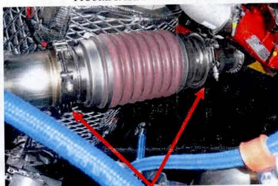
FIGURE 2. ISL DIESEL ENGINE
