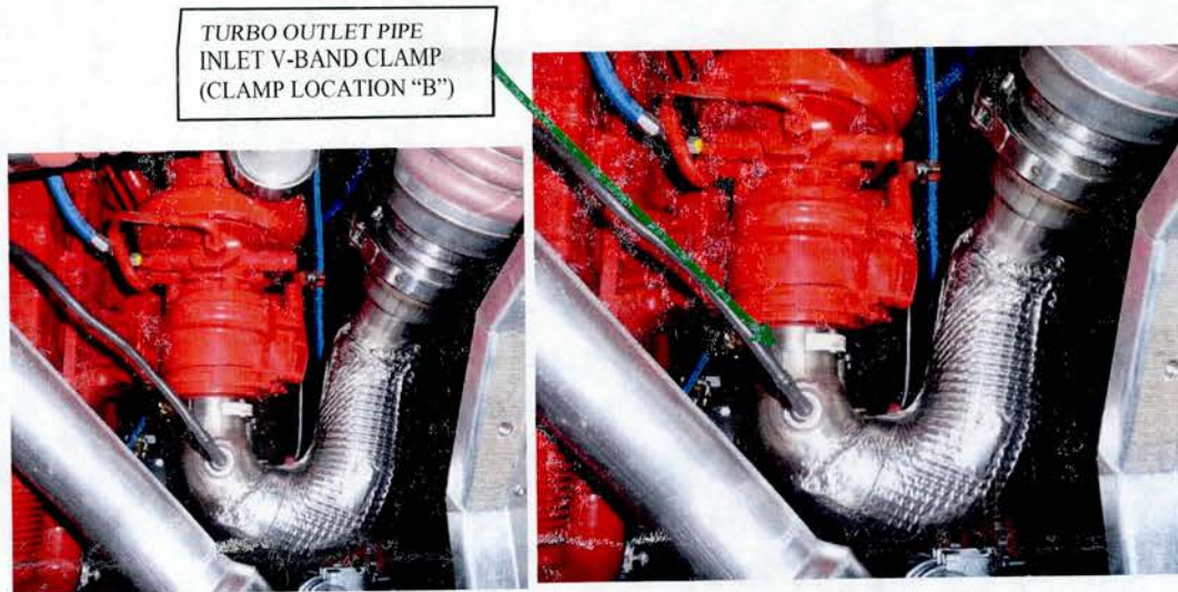
FIGURES 12 & 13. ISL-G CNG ENGINE SHOWN
