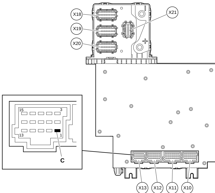
Fig. 3, SAM Cab (top view)
