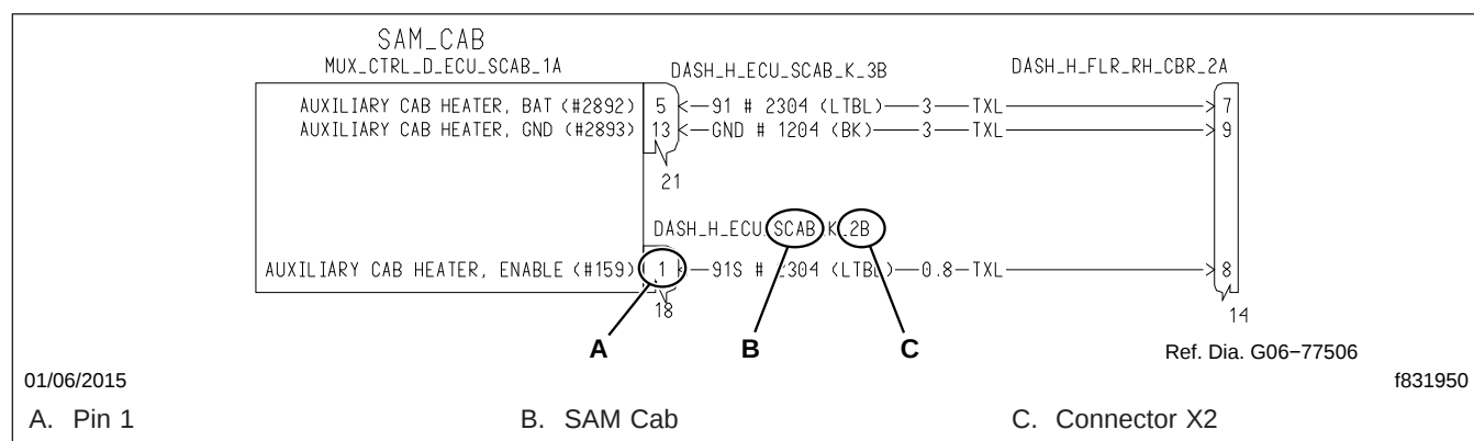
Fig. 1, Sample Schematic
