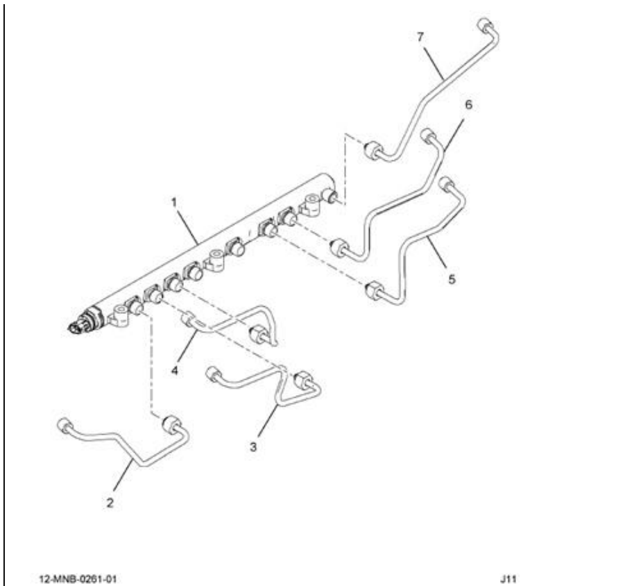
3014634C91 FUEL RAIL AND TUBE KIT, SPECIAL
