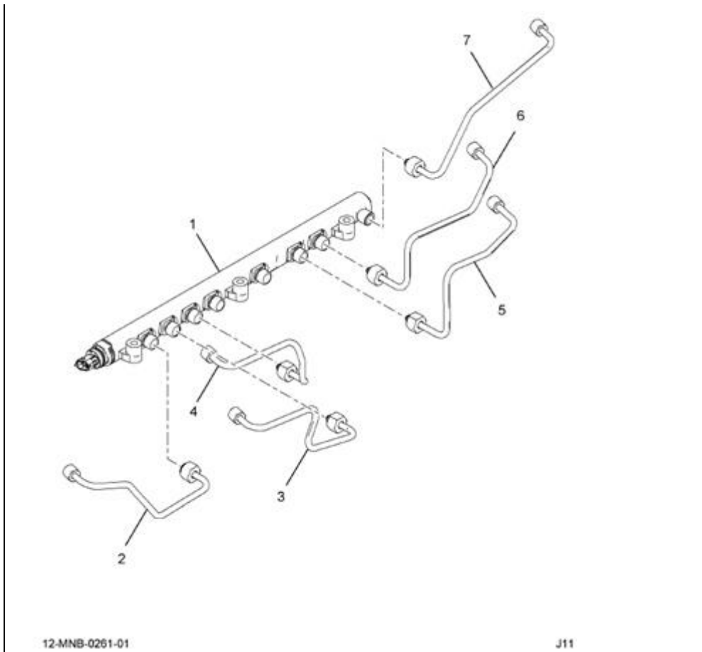
3014634C91 FUEL RAIL AND TUBE KIT, SPECIAL
