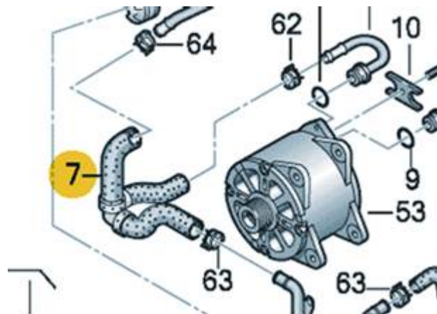
Figure 1. Connector hose (7).
