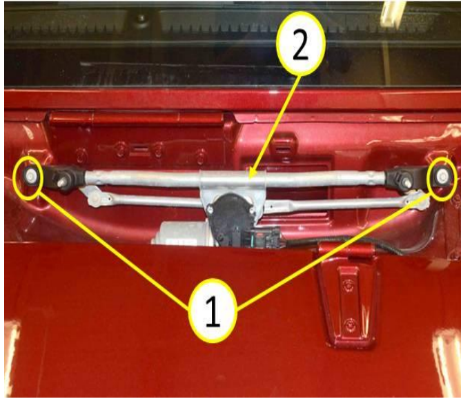
Fig. 1 Front Wiper Module
