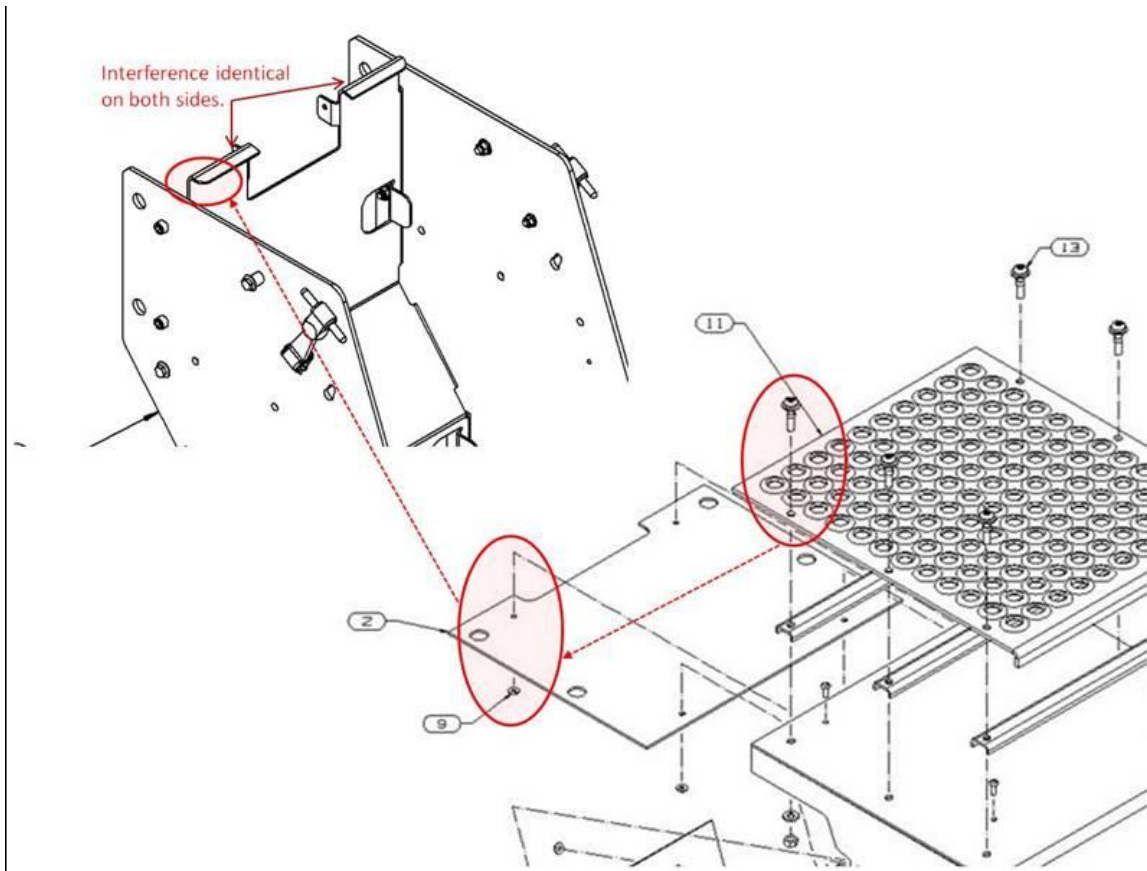
Figure 1 - Replace bolts causing the interference
