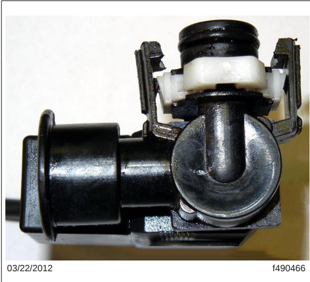
Fig. 1, 7-Watt Solenoid Valve ( 20±1 Ω)
