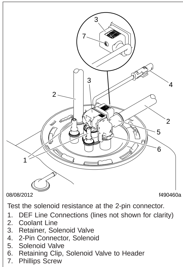
Fig. 4, DEF Coolant Flow Solenoid Installation (DEF lines not shown for clarity)
