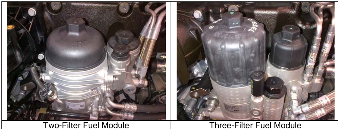
Figure 2 – DD Platform Fuel Filter Modules
