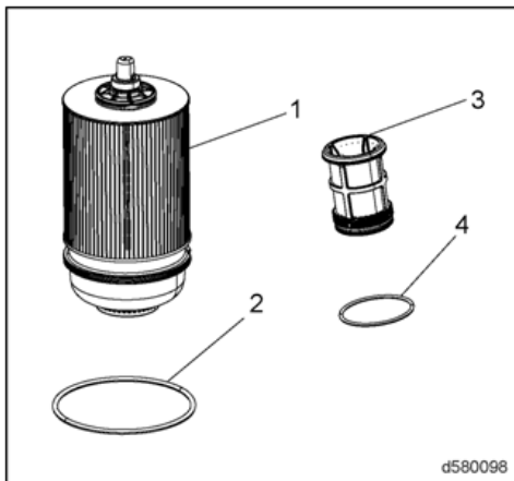
Figure 1 –Two-Filter Fuel Module Filter
