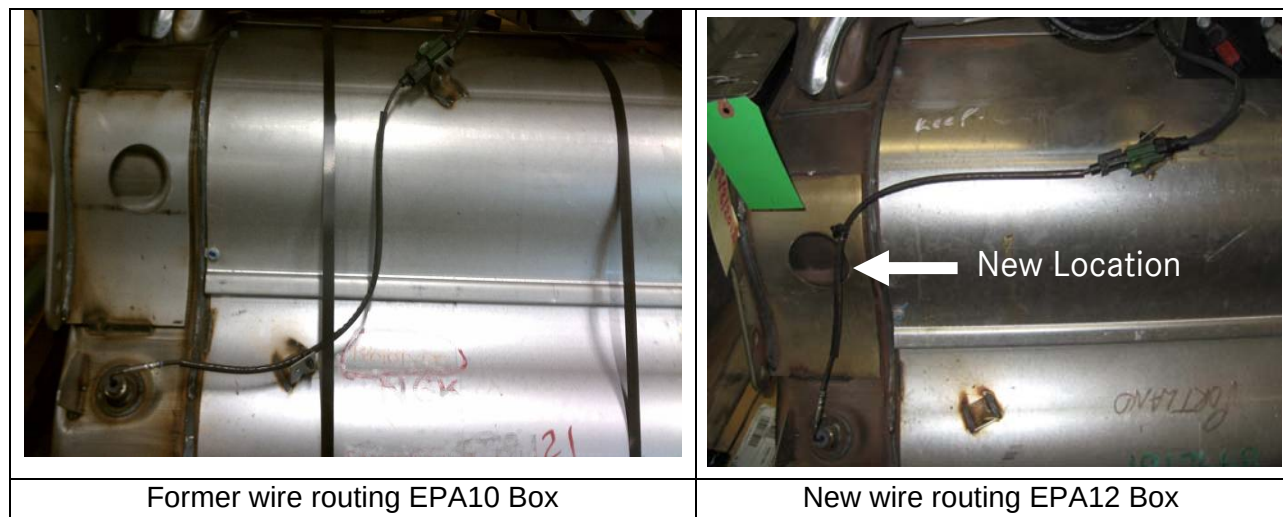
Figure 1 – Former EPA10 and New Temperature Sensors Wire Routing
