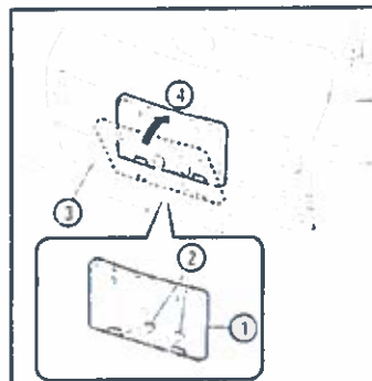
1 Mounting Bracket 2 Hooks 3 Air Intake 4 Rotate Bracket
