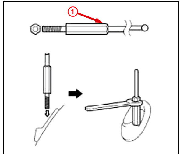
1 Hex-cut Type Antenna
