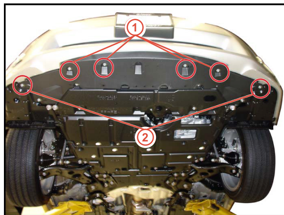
1 Self-Tapping Screws "A" (from Kit) 2 Self-Tapping Screws "B" (from Front Wheel Assy)
