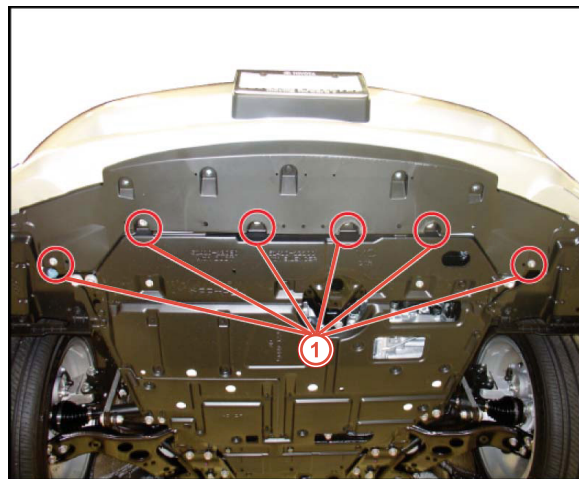
1 Bolts
