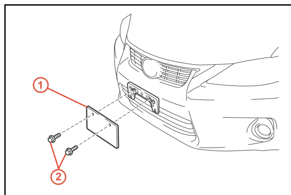
Figure 3. License Plate
