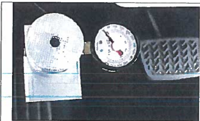
Brake pedal force gauge: SST 09709-00002
