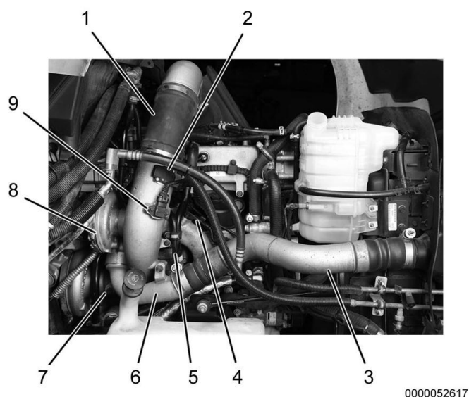
Figure 1. High-Pressure and Low-Pressure Turbochargers and Connections.
