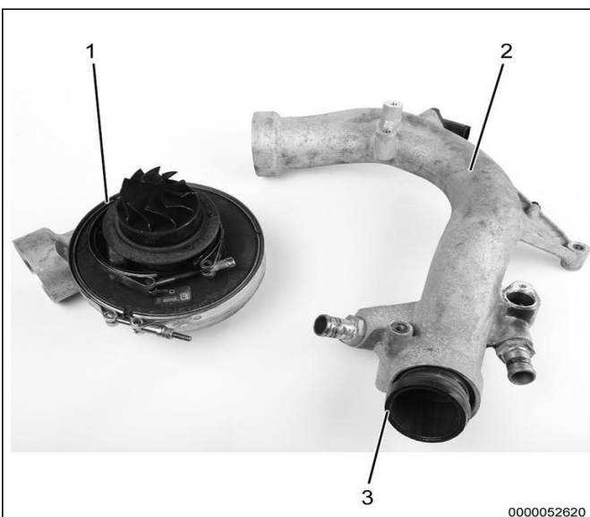
Figure 6. HP Turbocharger Center Cartridge and Air Supply Duct.
