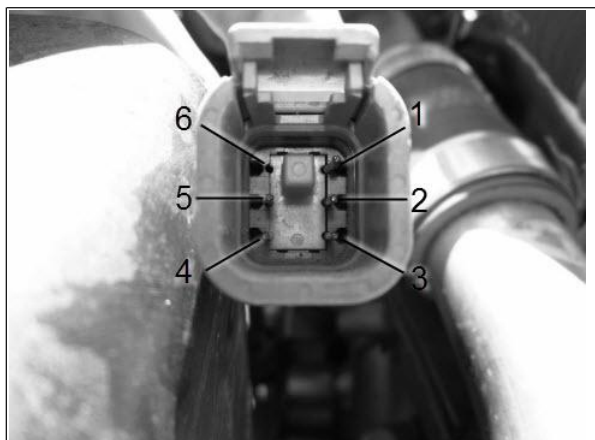
Figure 5. Pin Location Map (Front View)
