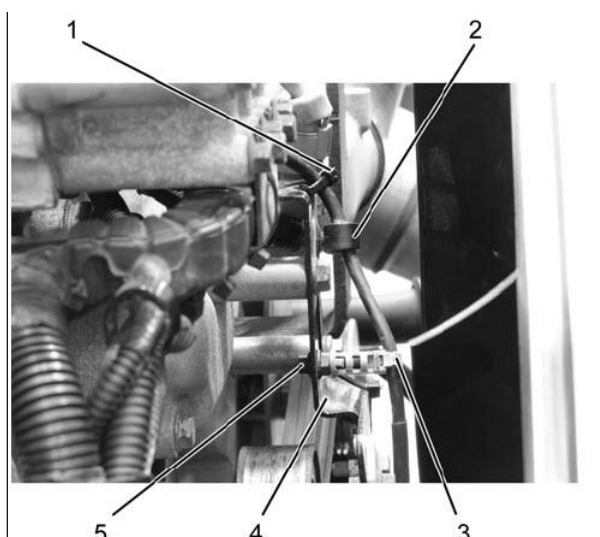
Figure 6. Fan Clutch Harness Reroute
