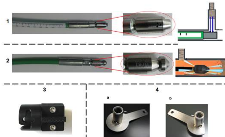
Figure 11. Special tool set VAS6825
