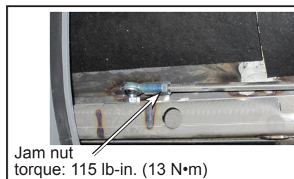
Figure 3 - Jam Nut Installation
