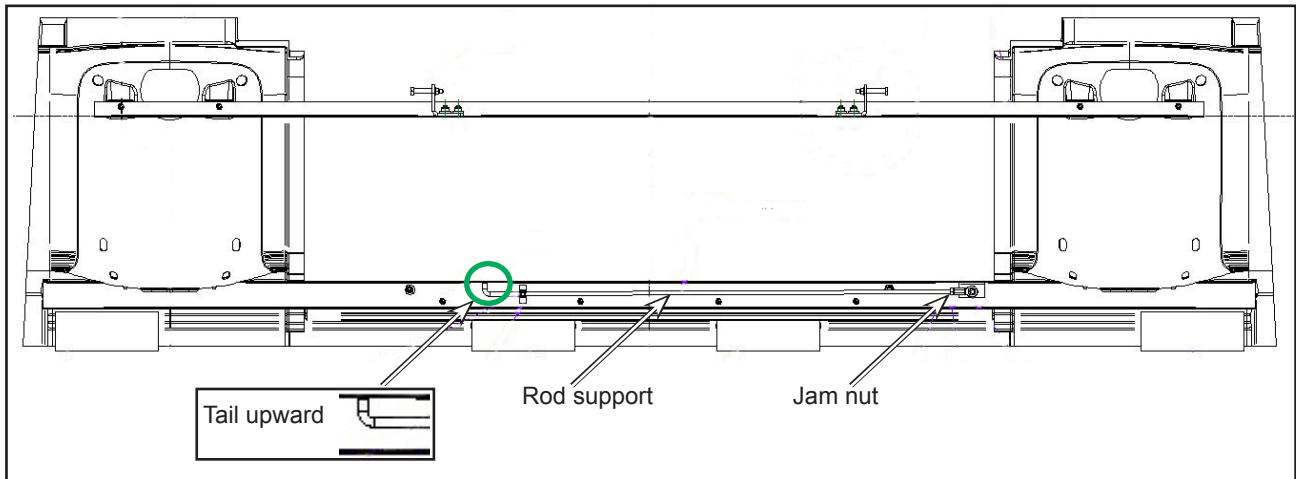
Figure 4 - Rear Seat Back View
