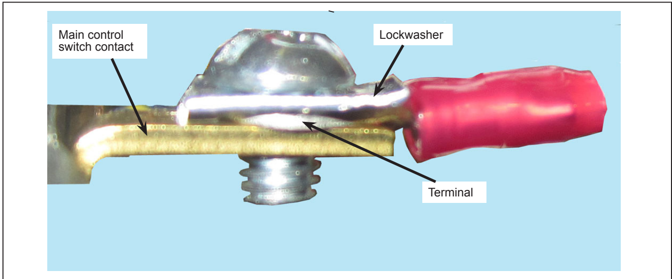
Figure 2 - Proper Installation of the Lockwasher and Terminal on the Contact
