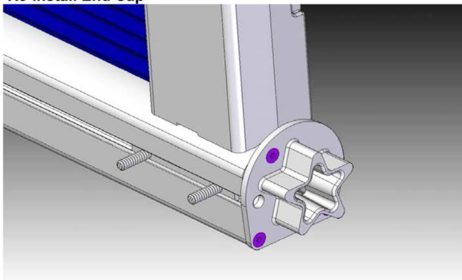
Figure 10 – Re-Install End Caps
