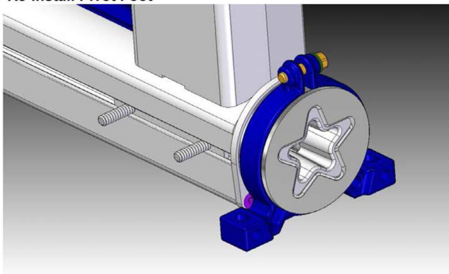
Figure 11 – Re-Install Pivot Foot
