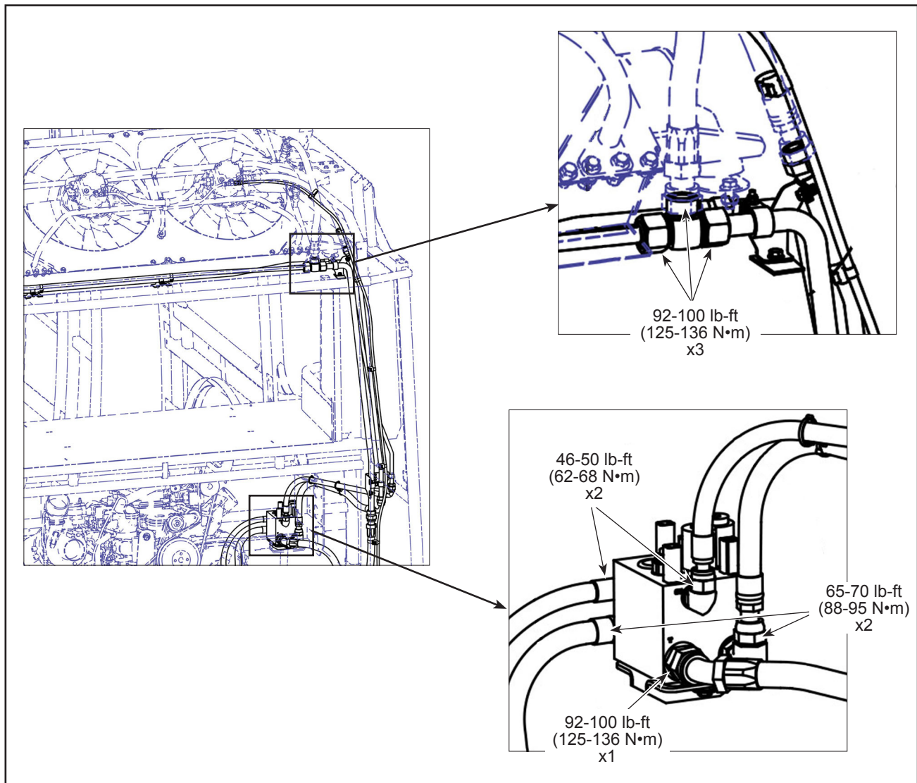
Figure 1 - Partial View of the Hydraulic System
