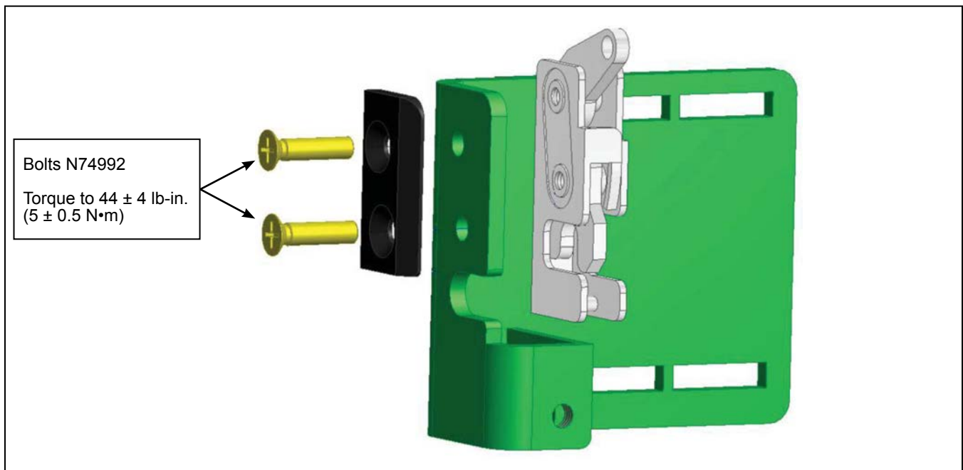
Figure 1 - Door Latch with Bolts N74992
