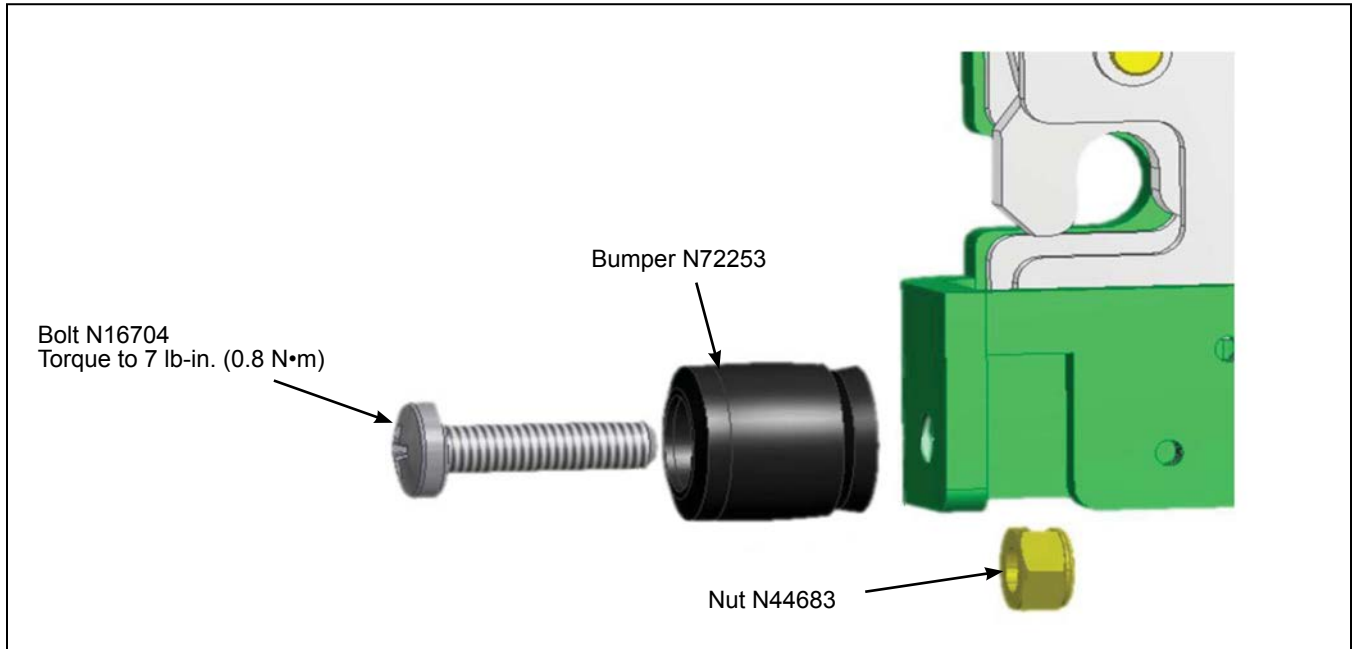
Figure 2 - Operator's door latch bumper N72253
