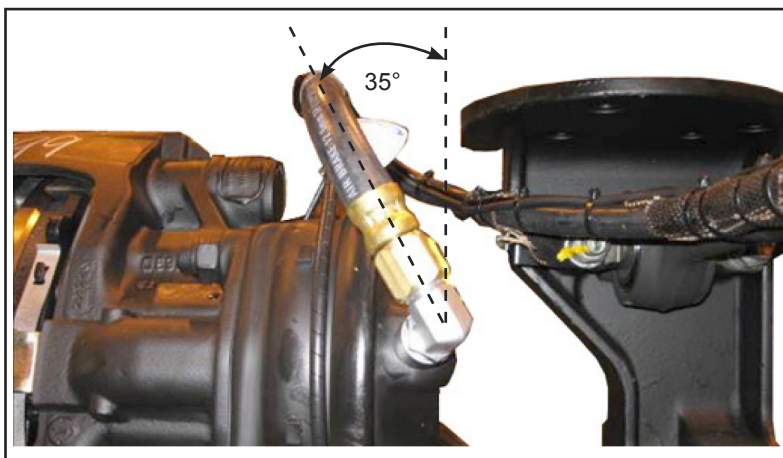
Figure 2 - 35° Brake Hose Angle
