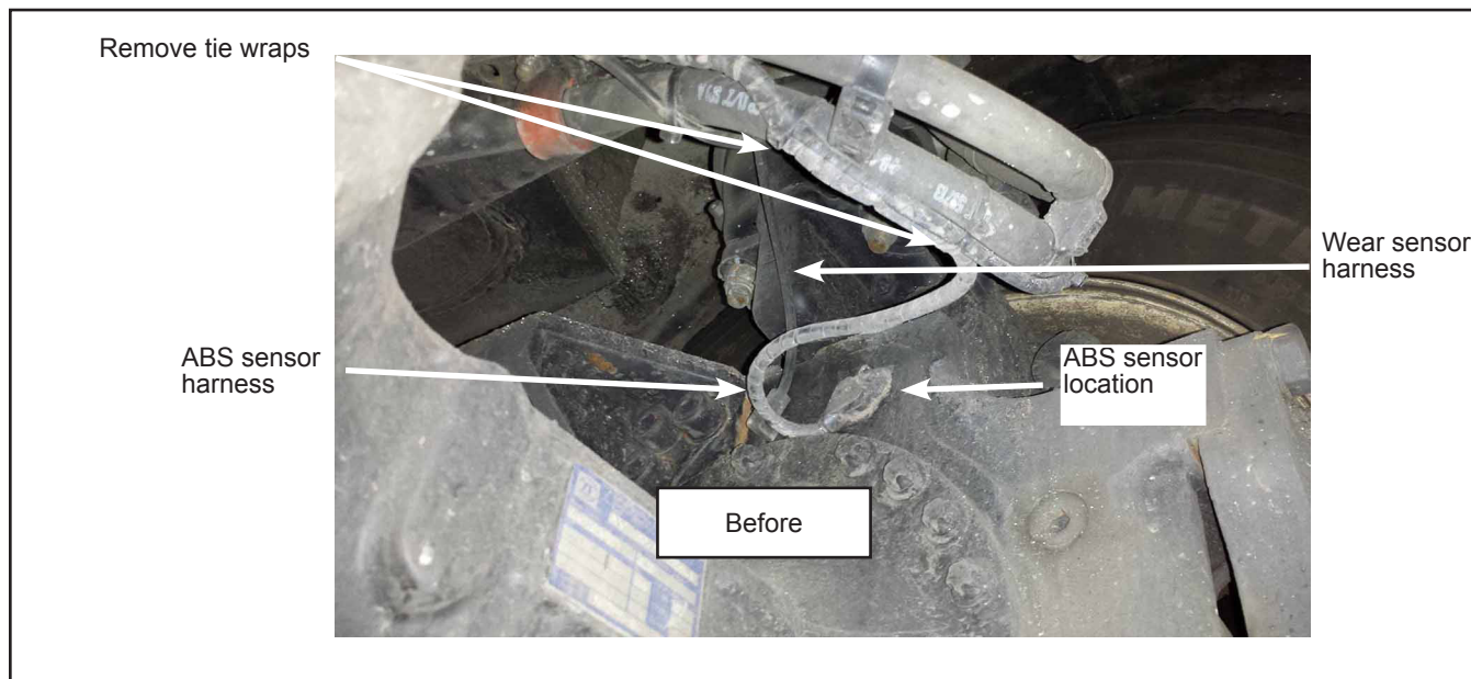
Figure 25 - Curb Side Electrical Harness Routing
