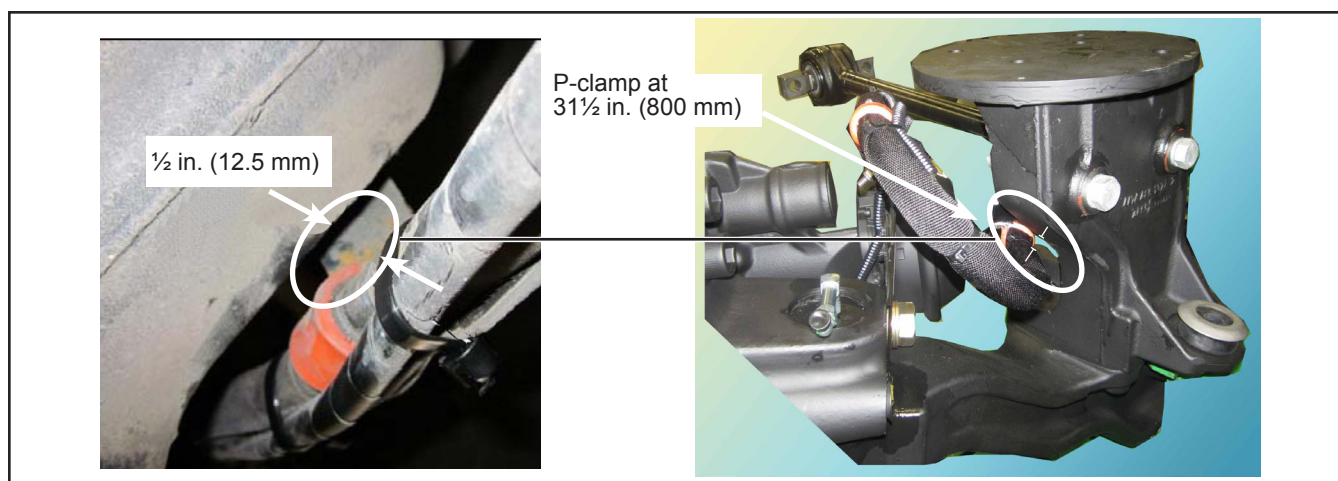
Figure 10 - Space Between the Brake Hose and the Axle
