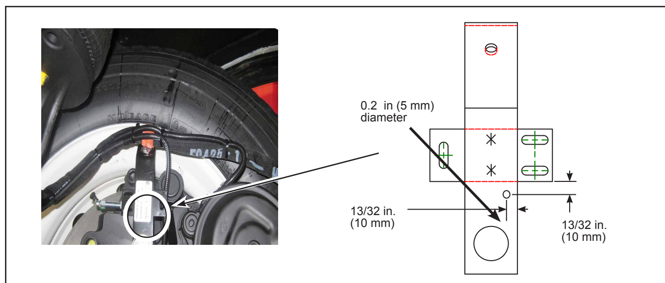
Figure 13 - Drilling of N20455-2 Support
