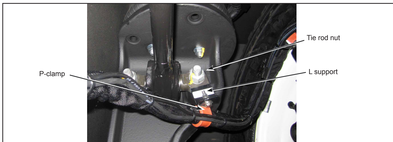
Figure 6 - P-Clamp Mounting
