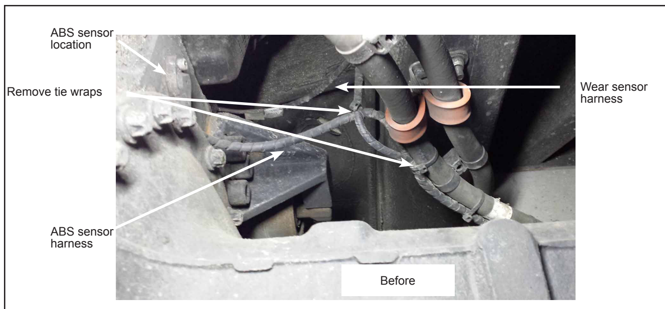
Figure 22 - Driver Side Electrical Harness Routing
