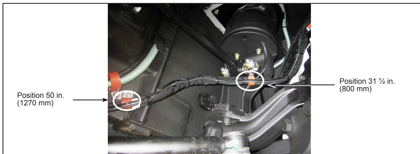
Figure 4 - P-Clamp Location on hose
