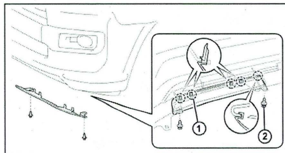
1 Claw 2 Clip
