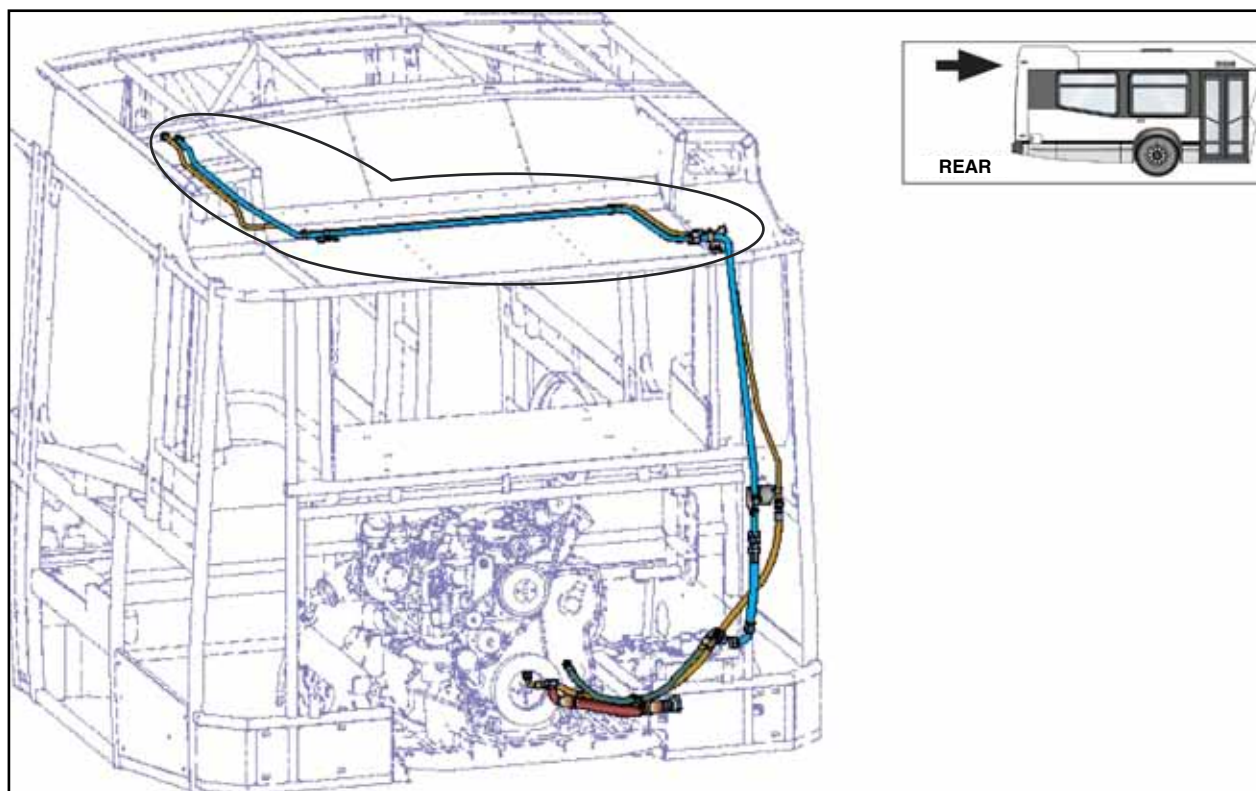
Figure 1 - Diagram of the Hydraulic system (typical)
